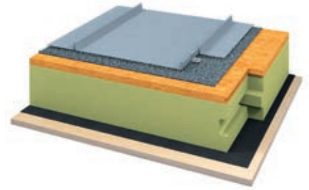
Fig. 2: Sealed roof build-up with double lock standing seam, with VAPOZINC on Linitherm PAL OSB insulation
