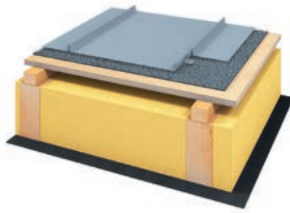
Fig. 1: Ventilated roof build-up with double lock standing seam, with VAPOZINC on 18 mm plywood
