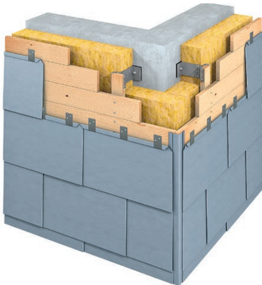
Outside corner/timber-metal-substructure (Example with tile size 333/600 mm)
