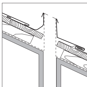
Penetration detail: Front flashing/back gutter, page 53
