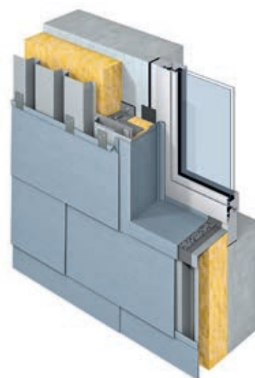
Window reveal/ Metal-substructure
