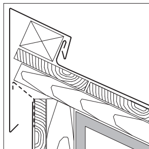
Ridge detail: monopitch roof page 52
