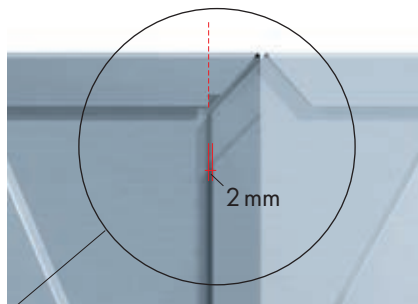
Base connection The crystal tiles are suspended in the prefabricated base profile.
