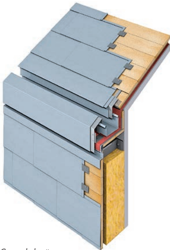
Concealed gutter
