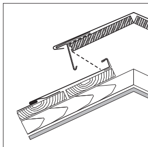
Ridge detail: gable roof page 52
