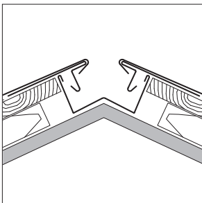
Hip detail flush, page 57
