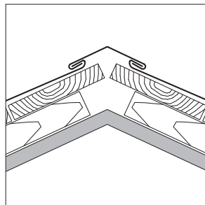
Hip detail with cap, page 57
