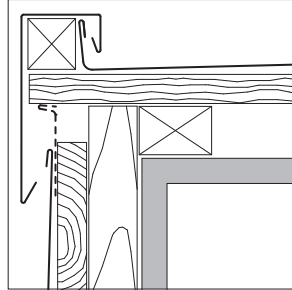
Verge detail: with flashing, page 55
