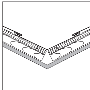
Valley detail: flush, page 56
