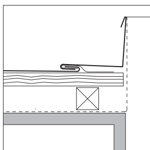
Penetration detail: Lateral connection, page 53
