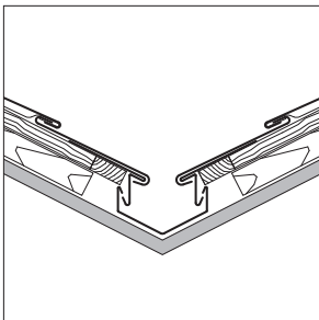
Valley detail: recessed, page 56
