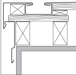
Verge detail: with verge gutter, page 55
