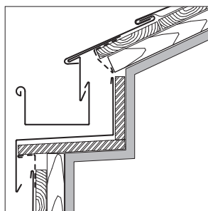
Eaves detail: Bracket-mounted gutter, page 54
