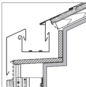
Eaves detail: Roof-integrated gutter, page 54
