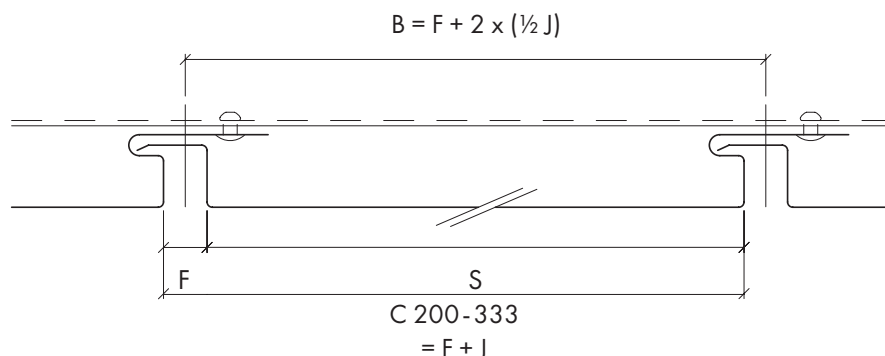
System section
