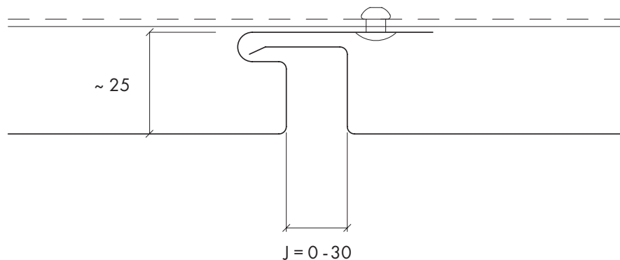
Joint configuration
