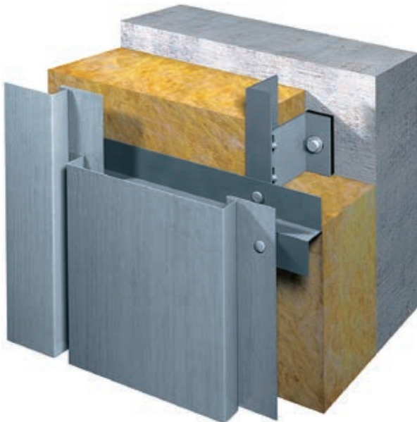
Multi-part substructure
