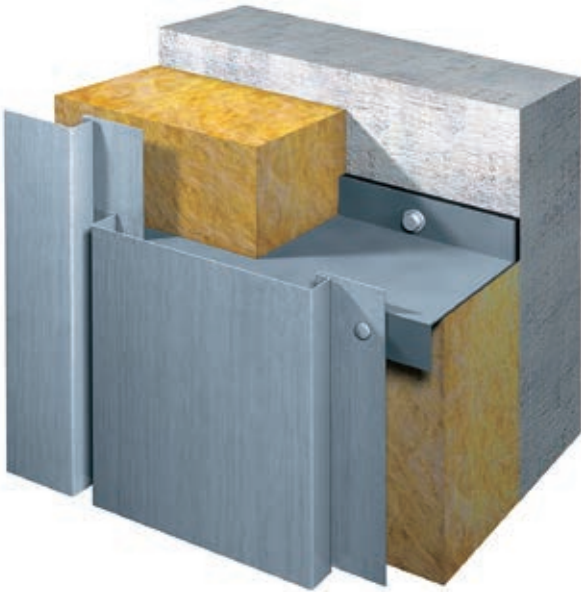
Single substructure
